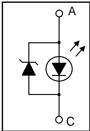
Internal circuit
