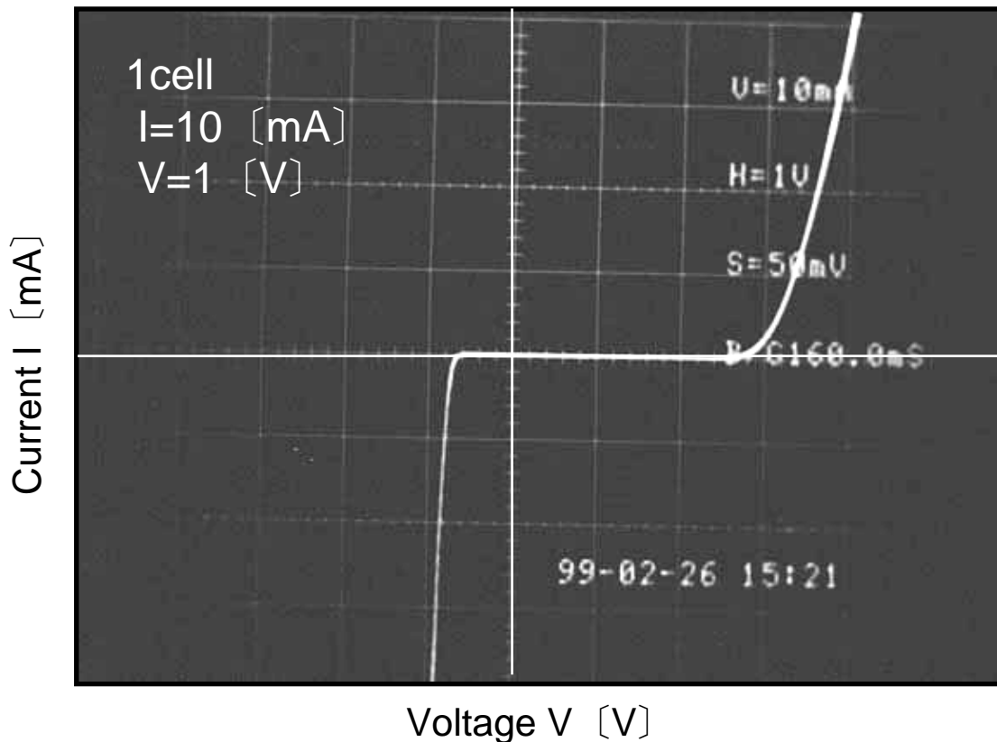
Current-Voltage characteristics
