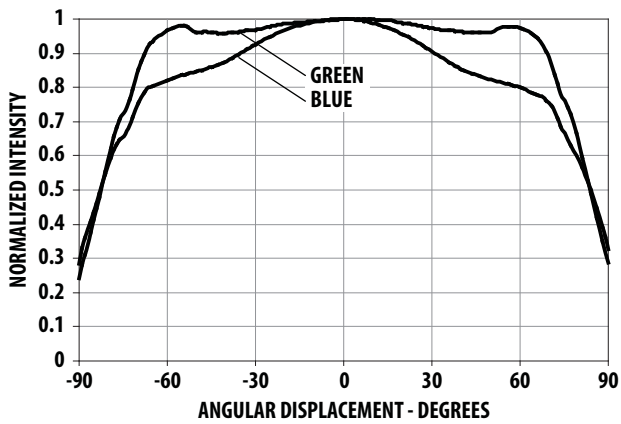
Figure 15. Radiation Pattern for Blue and Green.
