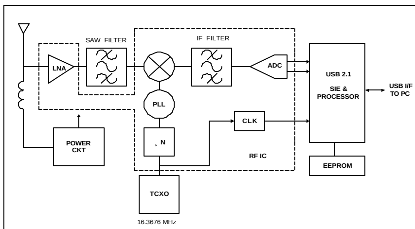
GPS1A Block Diagram
