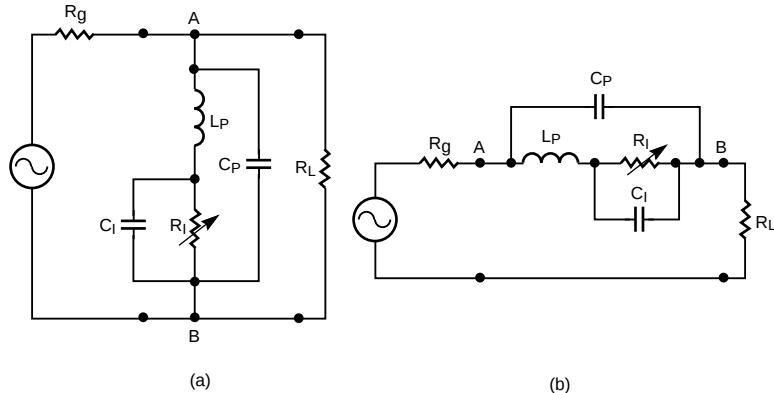
Figure 13. Resonant PIN Switches Realized with Use of Package Parasitics and Chip Capacitance.
