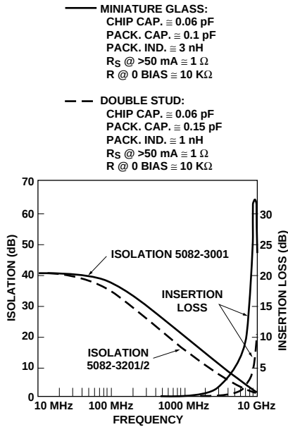
Figure 10(a). Attenuation of Series Diodes Used as a Switch in a 50 Ohm System.
