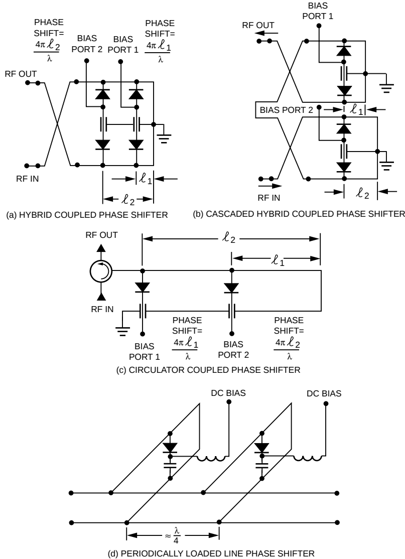
Figure 22. PIN Diode Phase Shifters.
