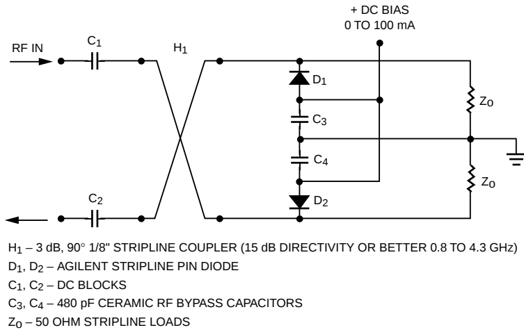
Figure 17. S-Band Single Hybrid Coupled PIN Attenuator.
