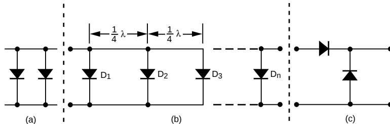
Figure 14. Reflective Mode Attenuators.
