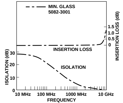
Figure 10(b). Attenuation of Shunt Diodes Used as a Switch in a 50 Ohm System.
