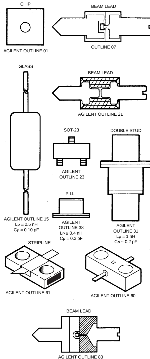
Figure 5. Package Outlines
