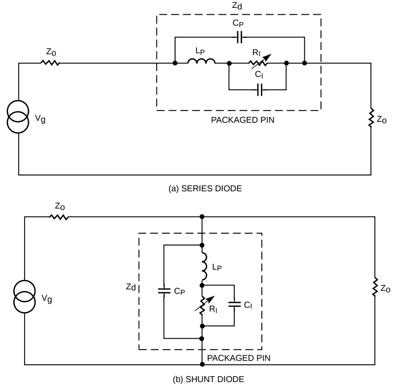
Figure 9. Packaged Diodes Used as Reflective Attenuators.
